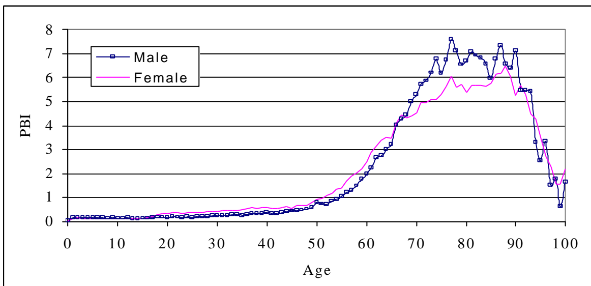
Figure 31: PBS Index
